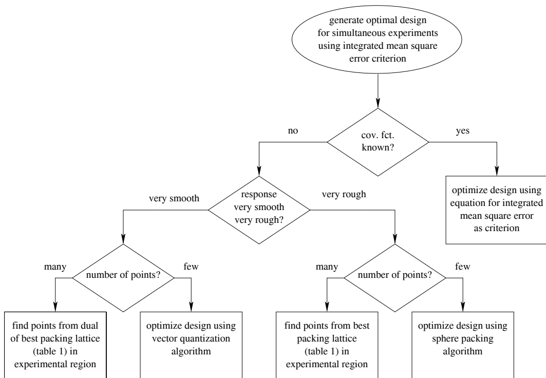
Figure 1.14: How to determine a suitable design method.
